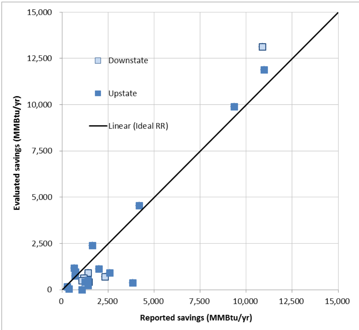
Figure 4-5. Reported and Evaluated Natural Gas Energy Savings by Region (NYSERDA)
